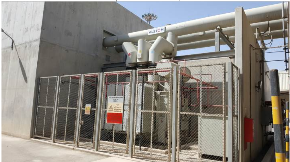
Adequate Segregation & Fire Protection of Oil-Filled Transformers Courtesy of SOHAR Aluminium LLC
