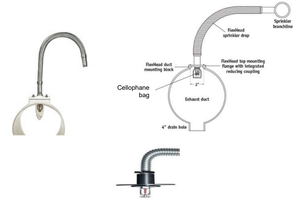
Fig. 2 - Examples of flexible sprinkler connections Posted and reprinted with permission of FM Global. ©2016-2017 Factory Mutual Insurance Company. All rights reserved.
