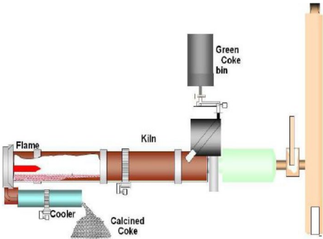
Courtesy of Aluminium Bahrain B.S.C. (Alba) – Calcination Plant & Marine Area
