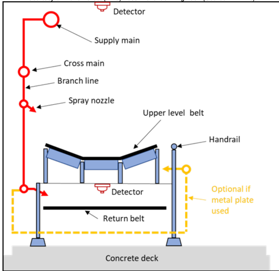
Typical conveyor belt protection (as per NFPA 15)
