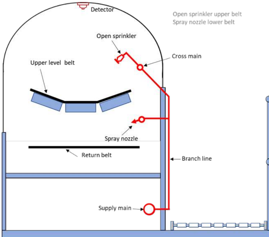
Typical hooded conveyor belt protection (as per NFPA 15)
