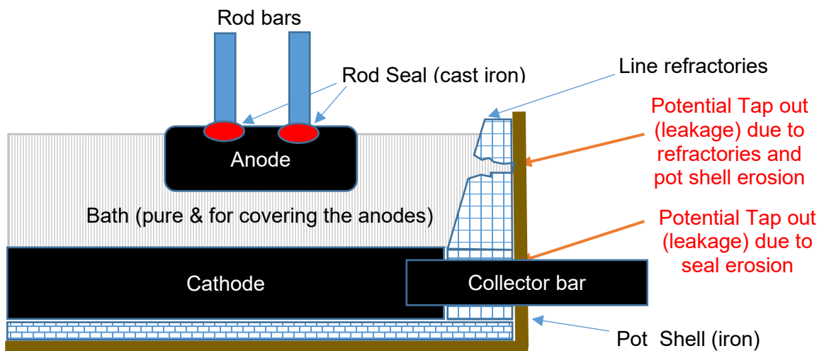
Pot Cross section view – not to scale
