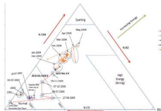
Figure 11 Progressive degradation of the insulation of a transformer following a series of geomagnetic storms
